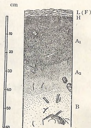
Fig. 4 Profile No. 4 BE-soil.
