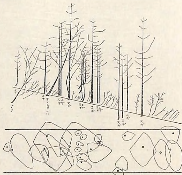
Fig. 3. Belt transect chart of forest near profile 1.
