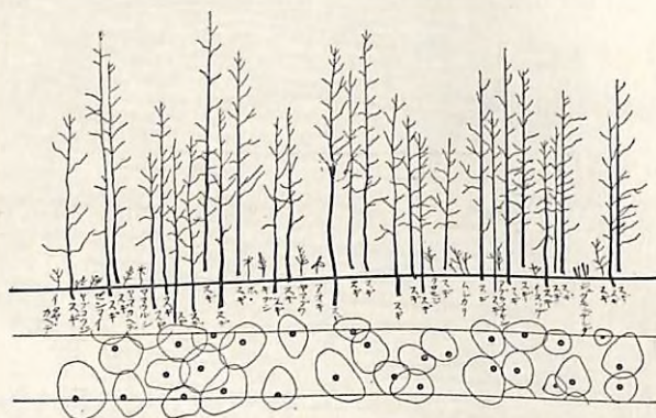
Fig. 21. Belt transect chart of forest near profile 10.
