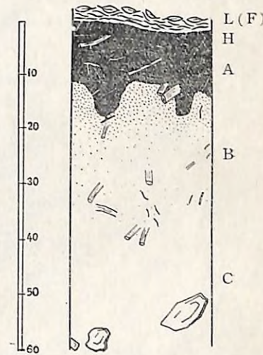
Fig. 5 Profile No. 5 BB-soil.
