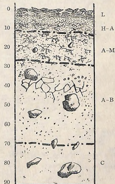
Fig. 1. Prof. No. 40. BA-soil.
