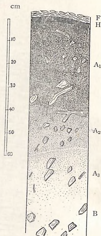
Fig. 6 Profile No. 6 BE-soil
