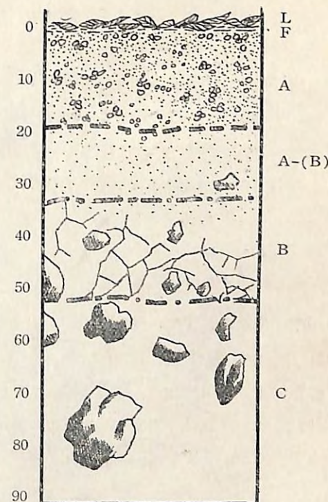
Fig. 6. Prof. No. 4. Bc-soil.
