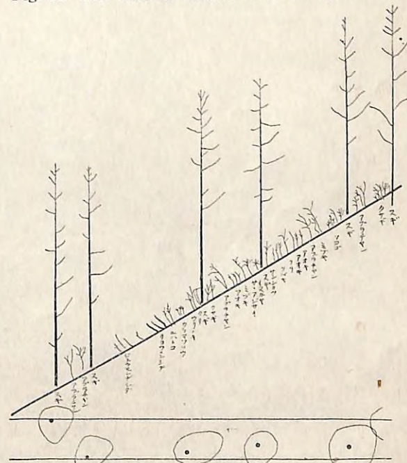
Fig. 33 Belt transect chart of forest near profile 17.
