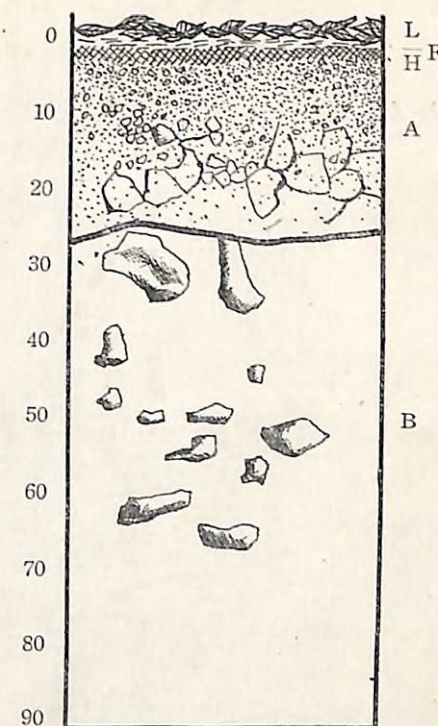
Fig. 3. Prof. No. 25. BB-soil.
