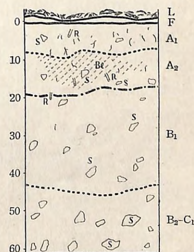
Fig. 26 Profile 13. B D -soil.
