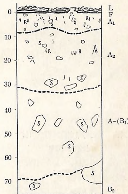
Fig. 16. Profile 8. BE (Br)-soil.
