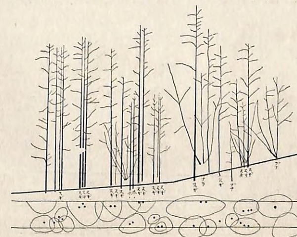
Fig. 13. Belt transect chart of forest near profile 6.
