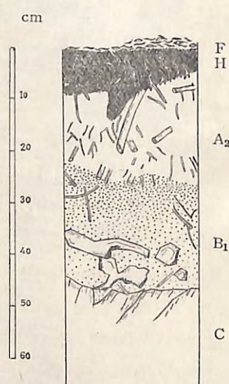
Fig. 1 Profile No. 1 PDI-soil.
