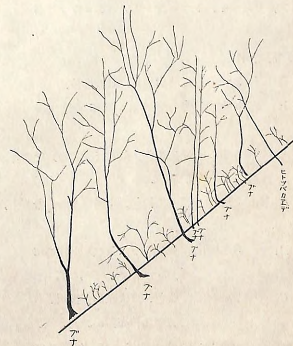
Fig. 5. Belt transect chart of forest near profile 2.
