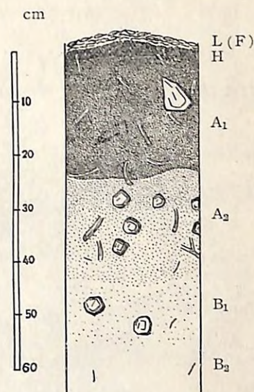
Fig. 2 Profile No. 2 BD-soil.
