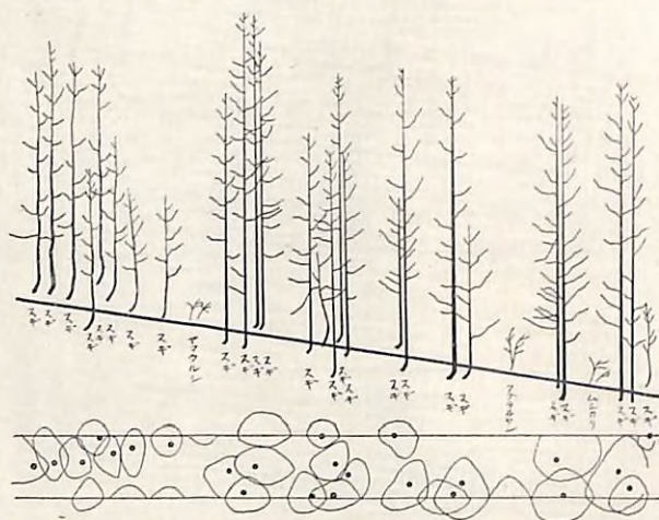
Fig. 27 Belt transect chart of forest near profile 13.
