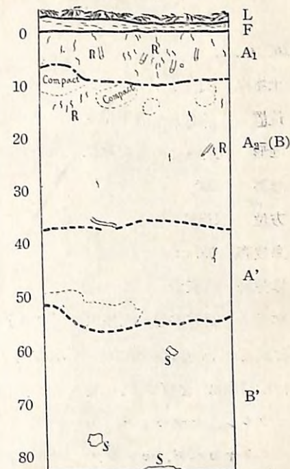
Fig. 22. Profile 11. BE (BF)-soil.
