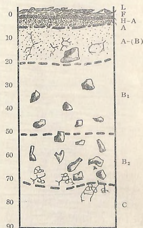
Fig. 5. Prof. No. 31. BB-soil.
