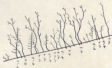
Fig. 7. Belt transect chart of forest near Profile 3.
