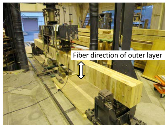
5-layer 7-ply CLT in the minor strength direction (5-7-Mi)
