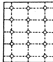
図5-3 SSUの配置 (○:SSU)
