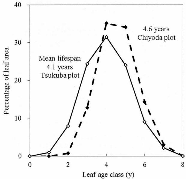
Fig. 4. Percentage of dead leaf area by leaf age class in withered small branch and leaf modules of Cryptomeria japonica var. japonica forests. Solid line and open diamond, 40-year-old stand in the Tsukuba plot (mean lifespan, 4.1 years); broken line and closed diamond, 19-year-old stand in the Chiyoda plot (mean lifespan, 4.6 years).
