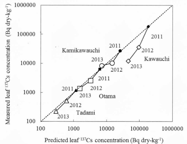
Fig. 8. Comparison of the chronosequential changes between predicted and measured leaf ^{137}\text{Cs} concentrations in Cryptomeria japonica var. japonica forests ◇, Kawauchi PSP; ○, Kamikawauchi PSP; □, Otama PSP; △, Tadami PSP. The broken line represents equal predicted and measured concentrations. Closed symbols (◆, ●, ■, ▲) represent the measured concentrations in 2011 (the first measurement).
